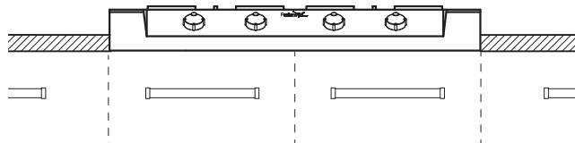
2. Sit-up installation on the cabinets and protruding over the worktop
